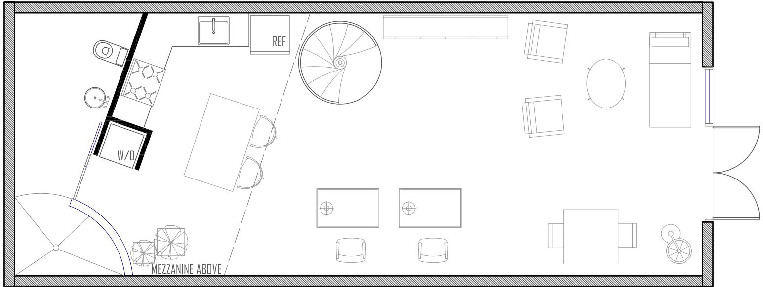
TYPE "A6" UNIT MAIN FLOOR
