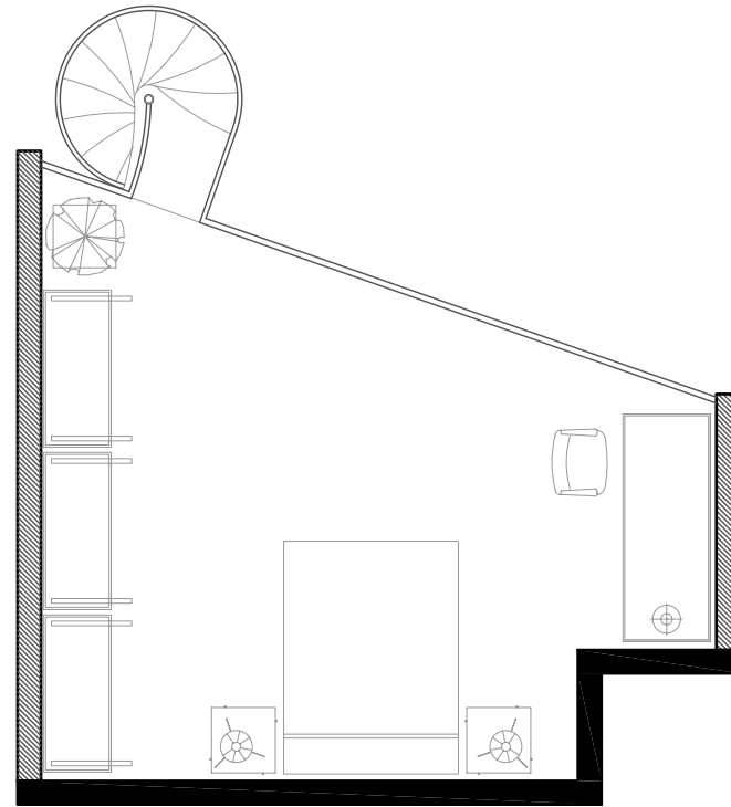
TYPE "A2" UNIT MEZZANINE
