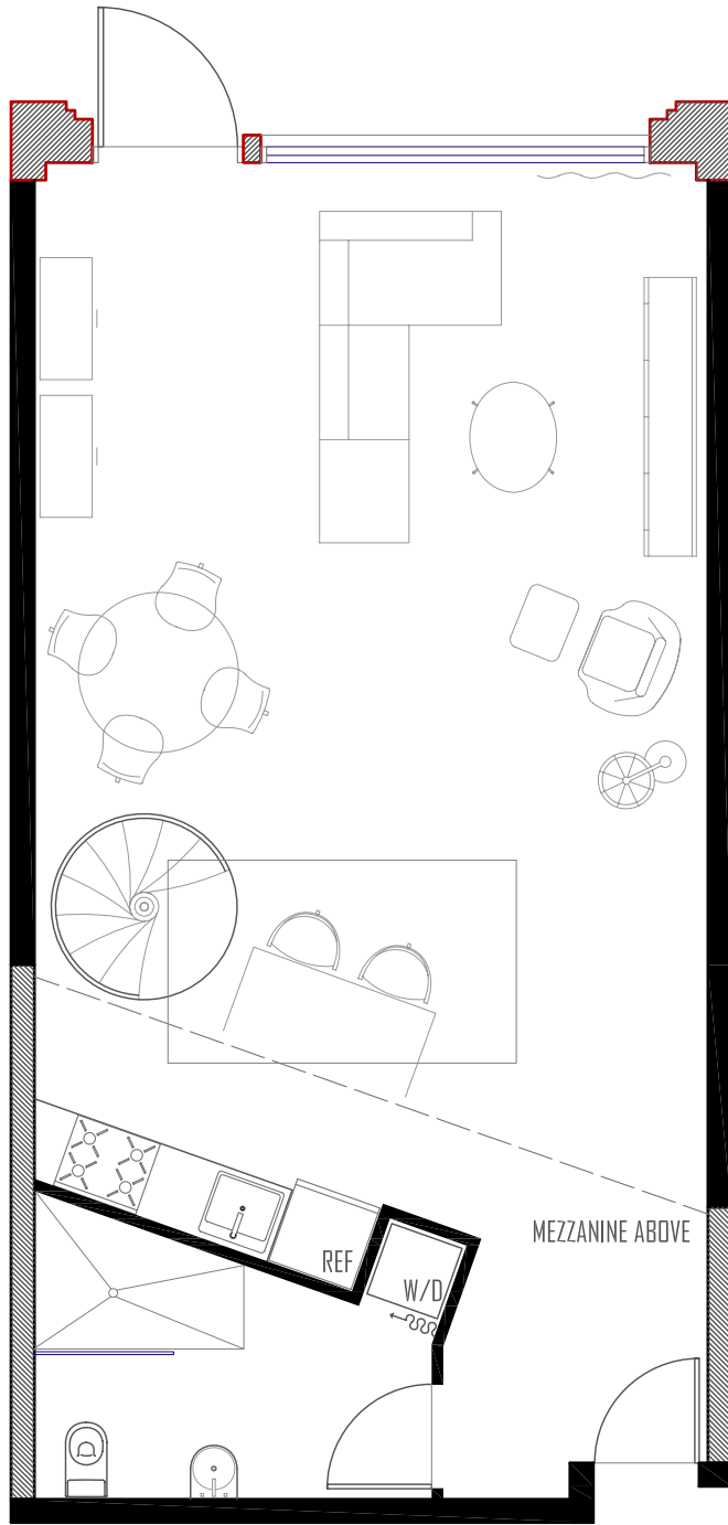
TYPE "A2" UNIT MAIN FLOOR
